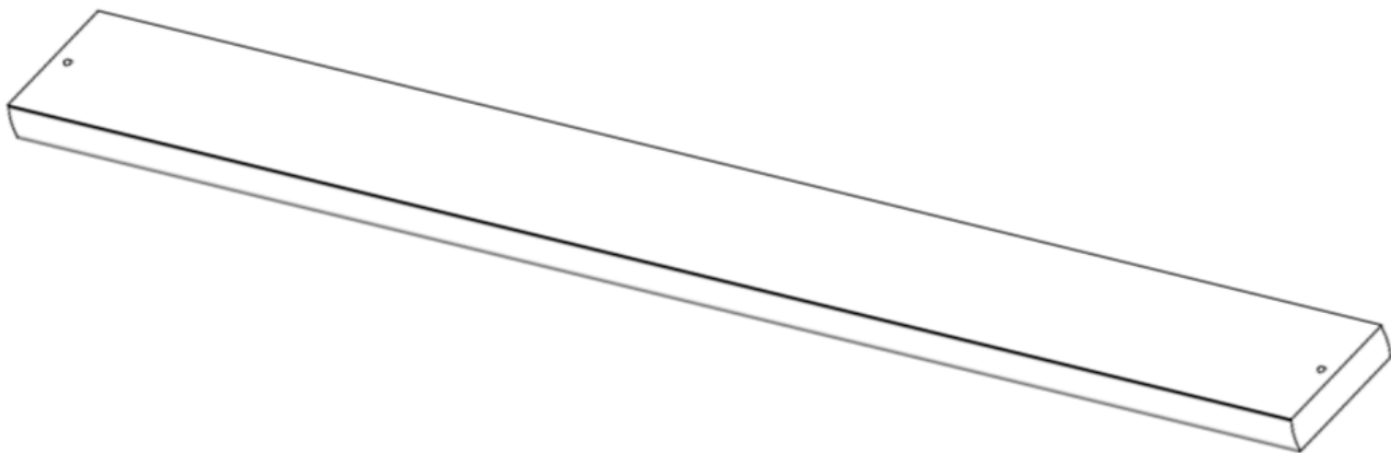
06 Lastro (680 x 69 x 17mm) x 12 un.
