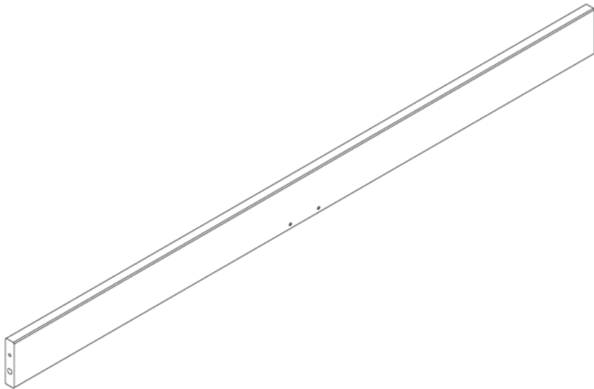
09 Travessa Peseira (1315 x 90 x 20mm)
