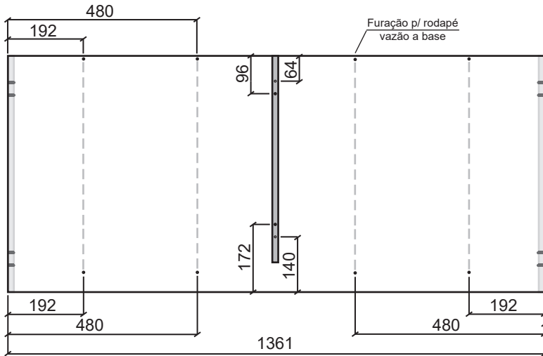
1. Base_Furação Interna_1361X600X15mm
