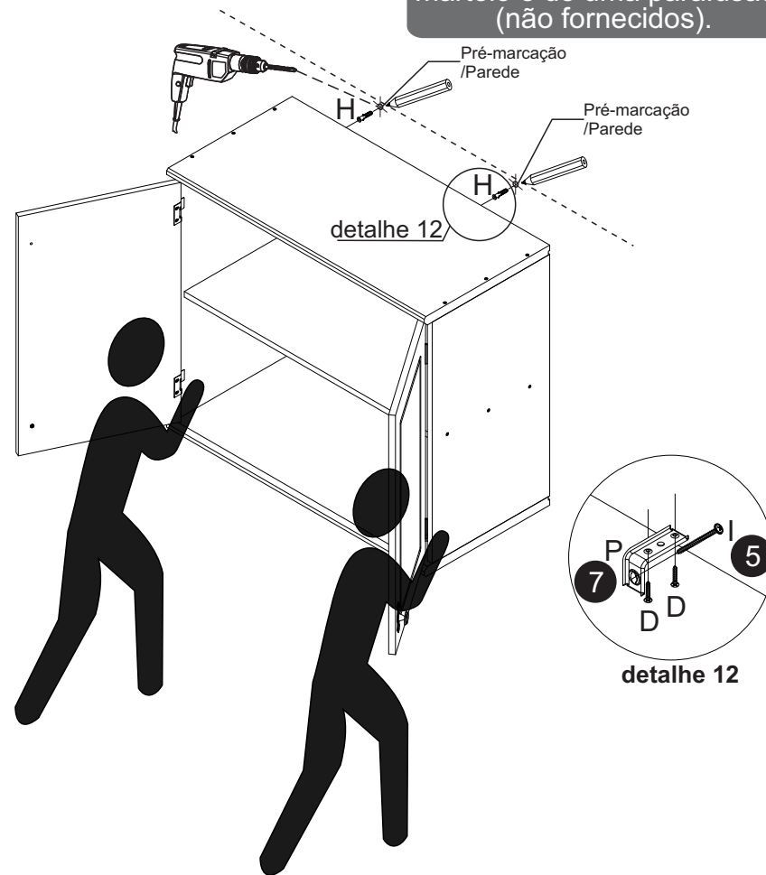
D- Parafuso FL PHS ZB 4,0x16mm (4x)
