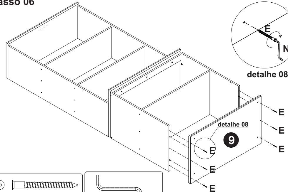
E- Parafuso Allen Soberbinho 5,0x50 mm (6x)
