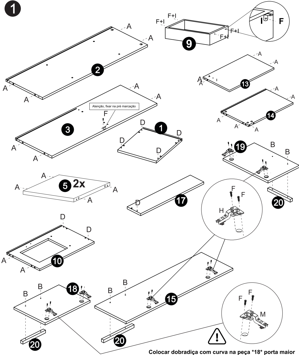
B - Parafuso 3,5x30 (31x)
