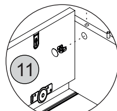
Detalhe 9 Detalle/Detail
