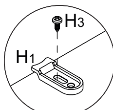
Detalhe 7 Detalle/Detail
