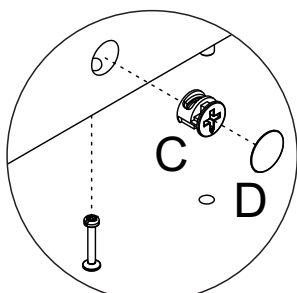
Detalhe 4 Detalle/Detail
