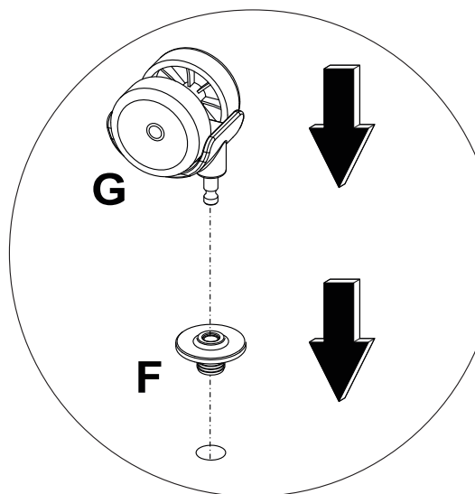
Detalhe 3 Detalle/Detail
