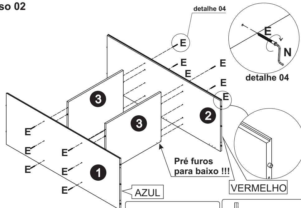
E- Parafuso Allen Soberbino 5,0x50 mm (12x)
