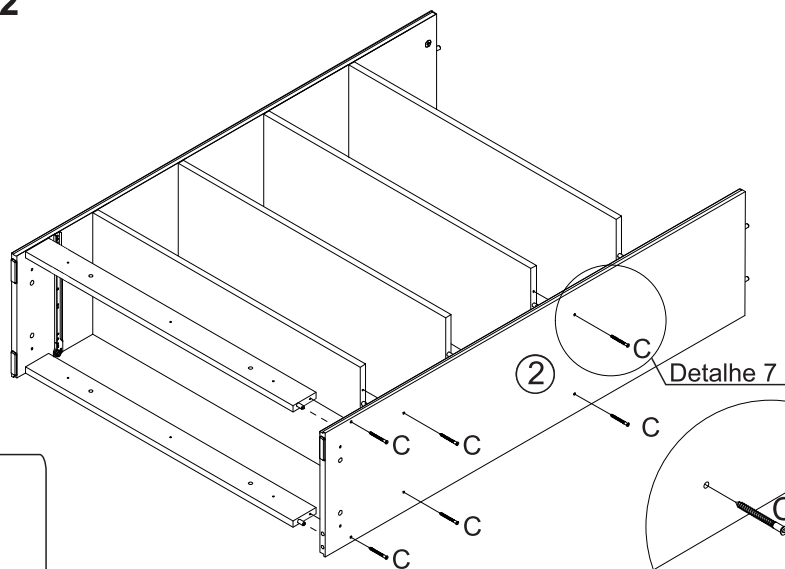
C- Parafuso Allen Soberbinho ZB 5,0X50mm Cab 7mm (6x)
