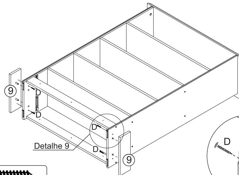
D- Parafuso FL PHS ZB 3,5X25mm (4x)
