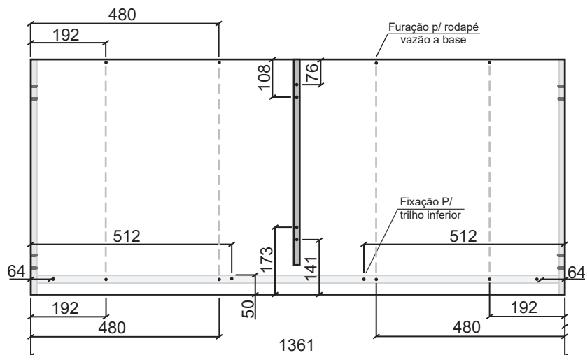
1. Base_Furação Interna_1361X600X15mm
