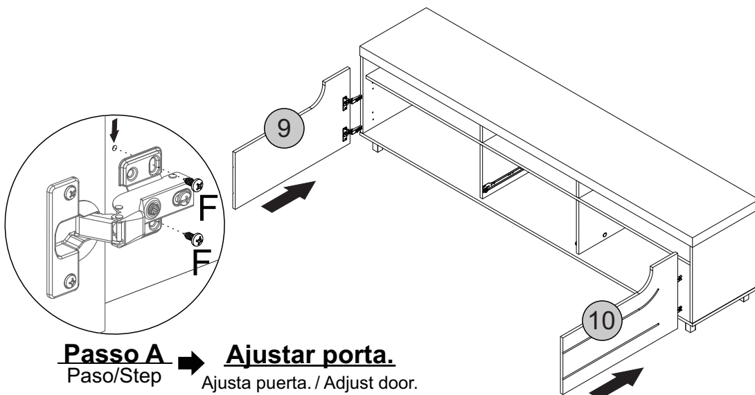
Detalhe 10 Detalle/Detail
