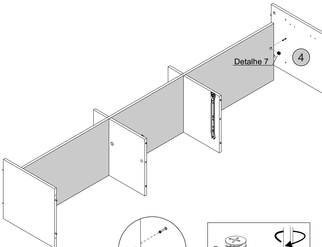
Detalhe 7 Detalle/Detail
