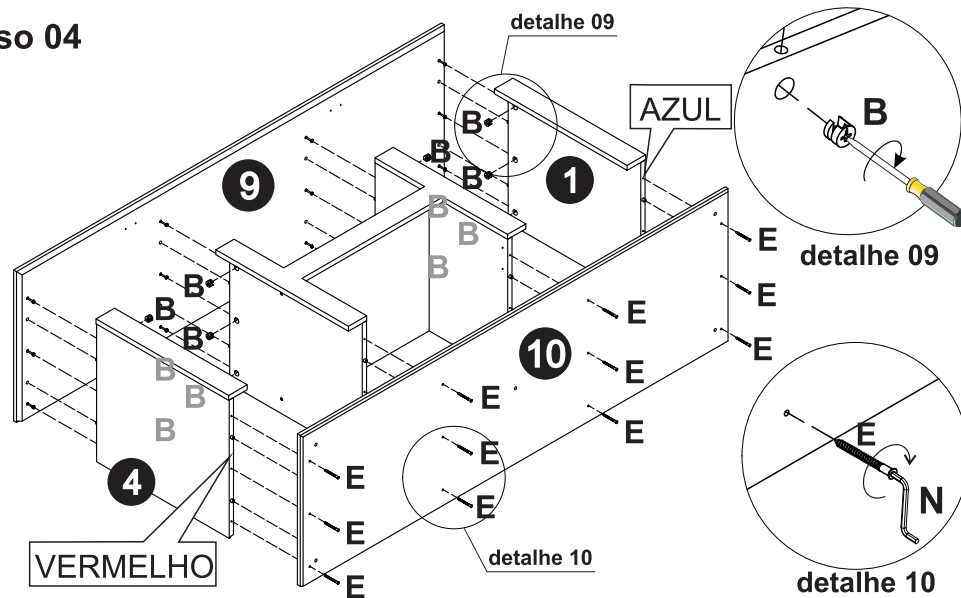
E- Parafuso Allen Soberbinho 5,0x50 mm (12x)
