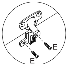
detalhe/detalle 1 (2x BEE051/3x BEE061)
