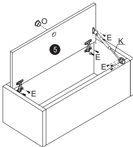
detalhe/detalle 1 (2x BEE051/3x BEE061)
