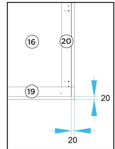
Top view for attaching the Upper Front Frame (19)
