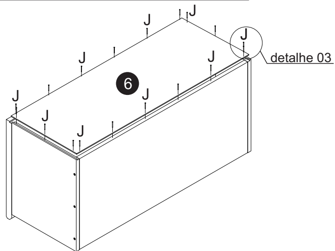
J- Pregos 10x10 (25x)
