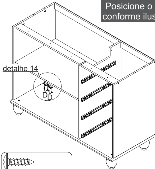
D- Parafuso FL PHS ZB 3,5x14mm (4x)
