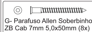
G- Parafuso Allen Soberbino ZB Cab 7mm 5,0x50mm (8x)
