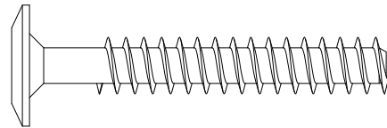
G- Parafuso Allen ZB 7,0X70mm Cab.13mm (5x) Cod 2821
