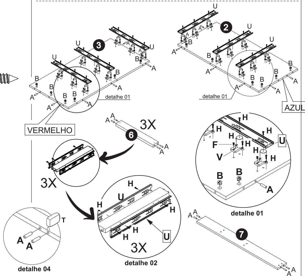
H- Parafuso CH PHS ZB 3,0x12 mm (72X)
