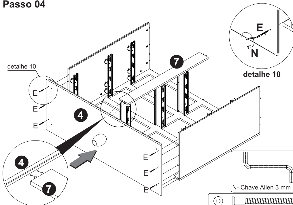
E-Parafuso Allen Soberbinho ZB 5,0x50 mm Cab Ø7 mm (6X)
