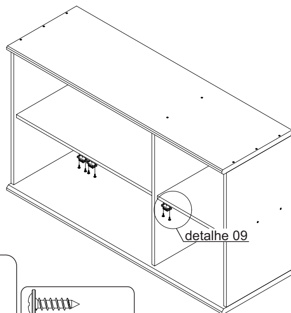
D- Parafuso FL PHS ZB 3,5x14mm (6x)
