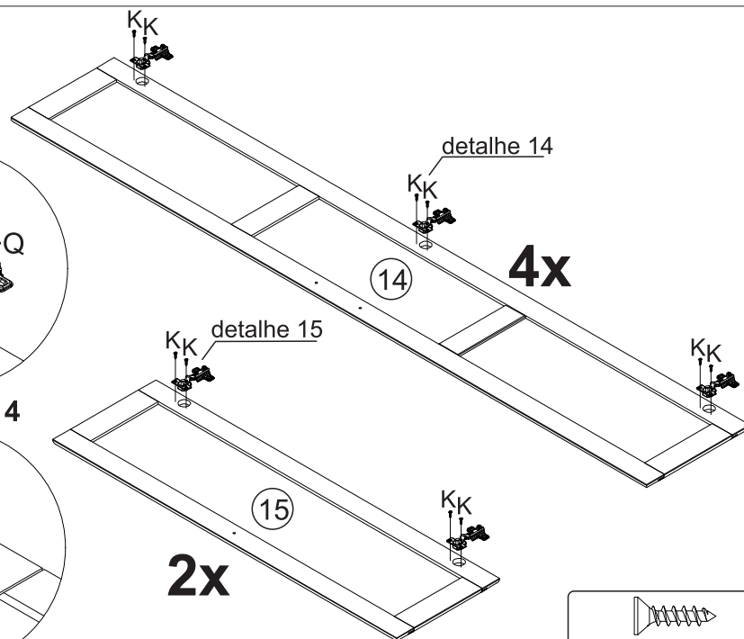
K-Parafuso CH PHS ZB 3,5X12 mm (32X)
