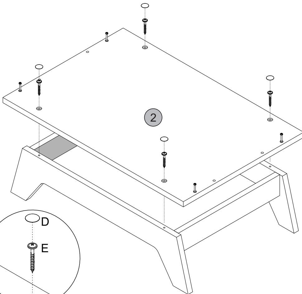
Detalhe 11 Detalle/Detail
