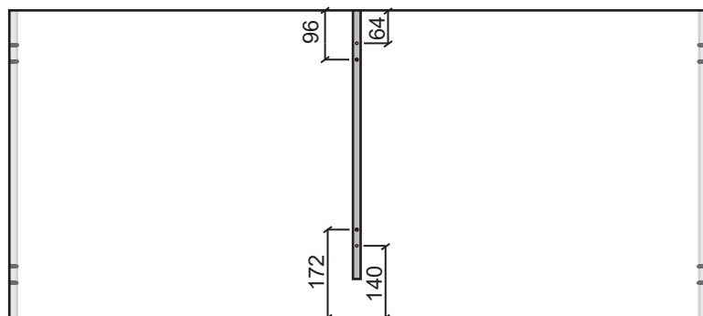
2. Chapéu_Furação Interna_1361X600X15mm
