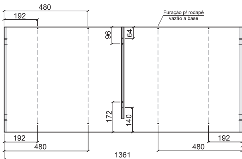
1. Base_Furação Interna_1361X600X15mm
