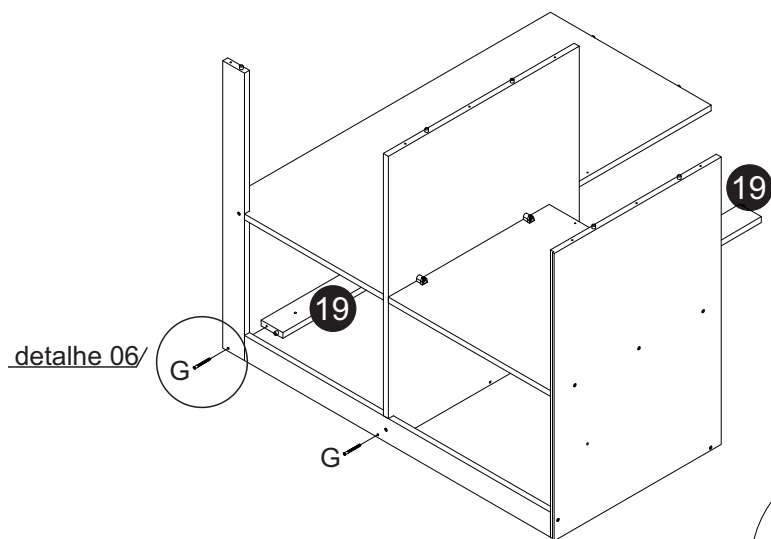
G- Parafuso Allen Soberbinho ZB 5,0X50mm Cab 7mm (2x)
