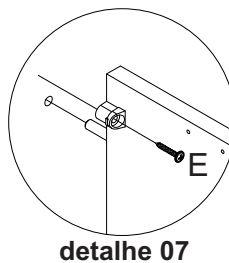
E- Parafuso FL PHS ZB 3,5x25mm (2x)
