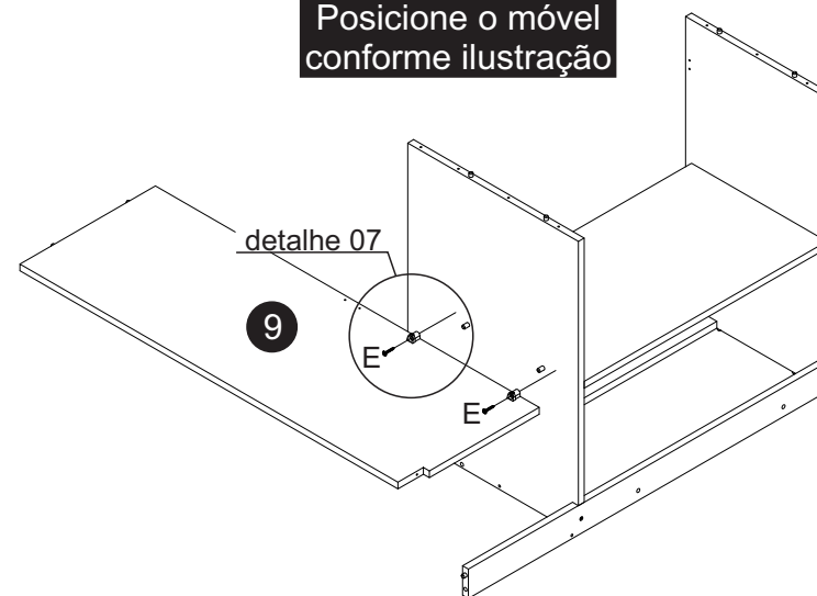
E- Parafuso FL PHS ZB 3,5x25mm (2x)
